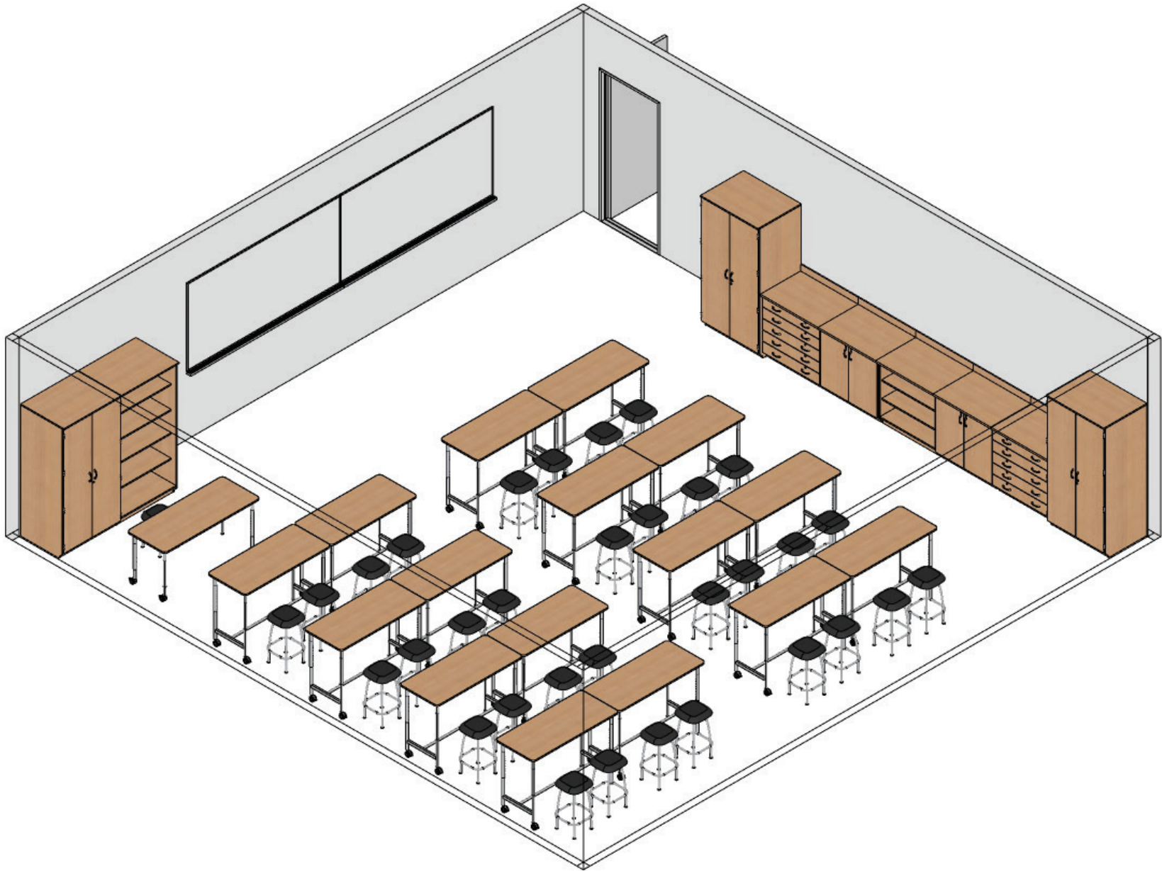
ISOMETRIC VIEW
