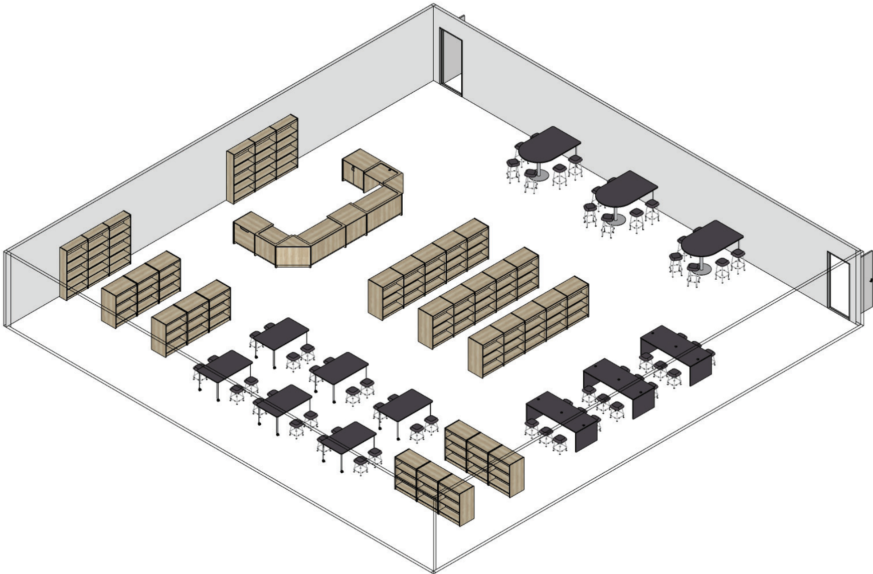
ISOMETRIC VIEW
